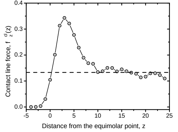
FIG. 6: Distribution of the force from the solid substrate acting on the liquid molecules in 0 \leq y \leq y_m = 2 , z_{cl} \leq z \leq z_{cl} + \lambda_{cl} in the case shown in Fig. 4 at U = 0:1 , \lambda_{12} = 0:9 . The dashed line indicates the mean background value.
