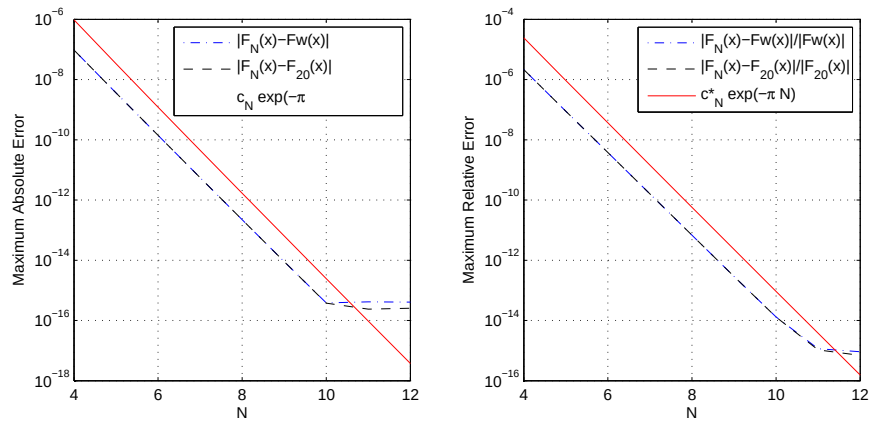
Fig. 1 Left hand side: maximum error, \max_{x \in [0, 2]} |F(x) - F_N(x)| , and its upper bound (12) (13), plotted against N , where F(x) is approximated by Fw(x) := e^{ix^2} w_{36}(e^{i\pi/4} x) with w_{36}(x) = 2
