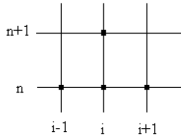
Figure 4.1: 2-D stencil representing nodes at n and n + 1 time levels, displaying an explicit timestep- ping approach.
