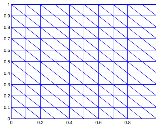
Figure 7.3: Delaunay triangulation of the unit square grid
