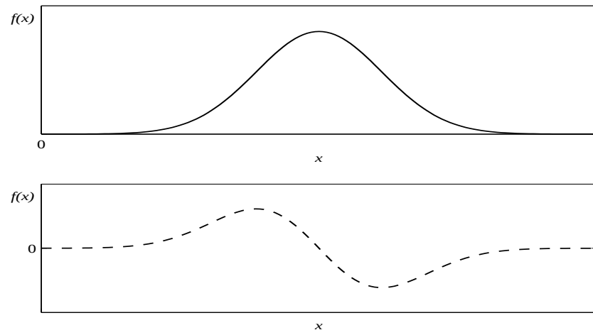
Figure 6.1: initial data (solid line) and its derivative (dashed line).
