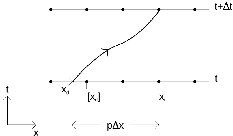
Figure 6.1: Ritchie's scheme
