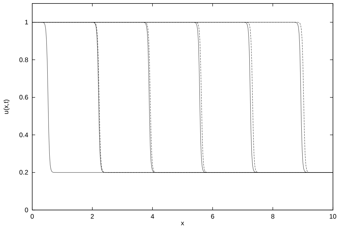
Figure 7.8: As Figure 7.7 but with 4 iterations of departure point scheme.
