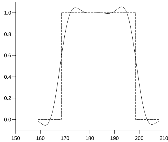
Figure 2.4: High order SL using cubic interpolation
