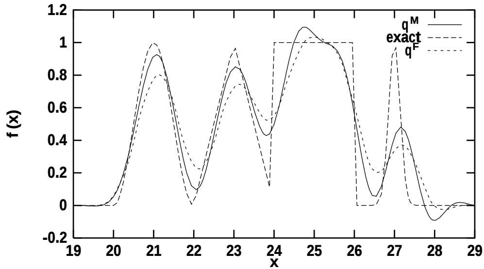
Figure 3.4: Comparison of mean and Fromm quadratic interpolants. Constant speed advection test over an irregular grid. Solutions shown after 1000 timesteps.
