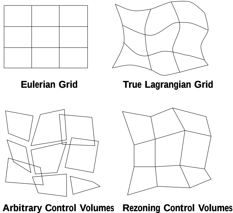
Figure 9.1: Control Volumes and Grids
