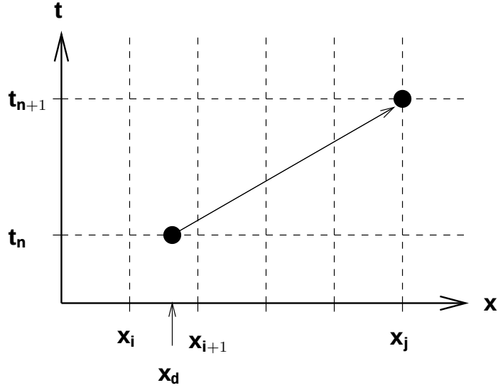
Figure 1.2: Basic SL method
