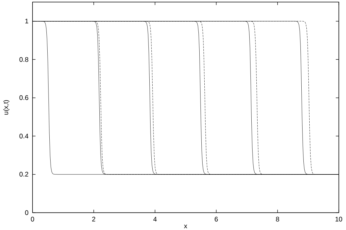
Figure 7.7: Moving front solution of viscous Burgers equation. Analytical solution (dashed lines) and SL solution (solid lines) after 0, 71, 142, 213, 284 and 355 steps. Mesh ratio \Delta t / \Delta x = 1.7 . Two iterations for calculating departure points.
