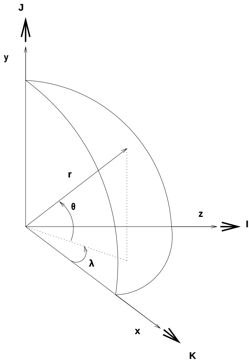
Figure 8.1: Geophysical spherical coordinates
