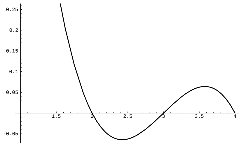
Figure 2.2: Lagrange basis function l_1
