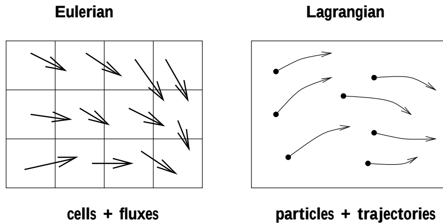
Figure 1.1: Eulerian and Lagrangian numerical models
