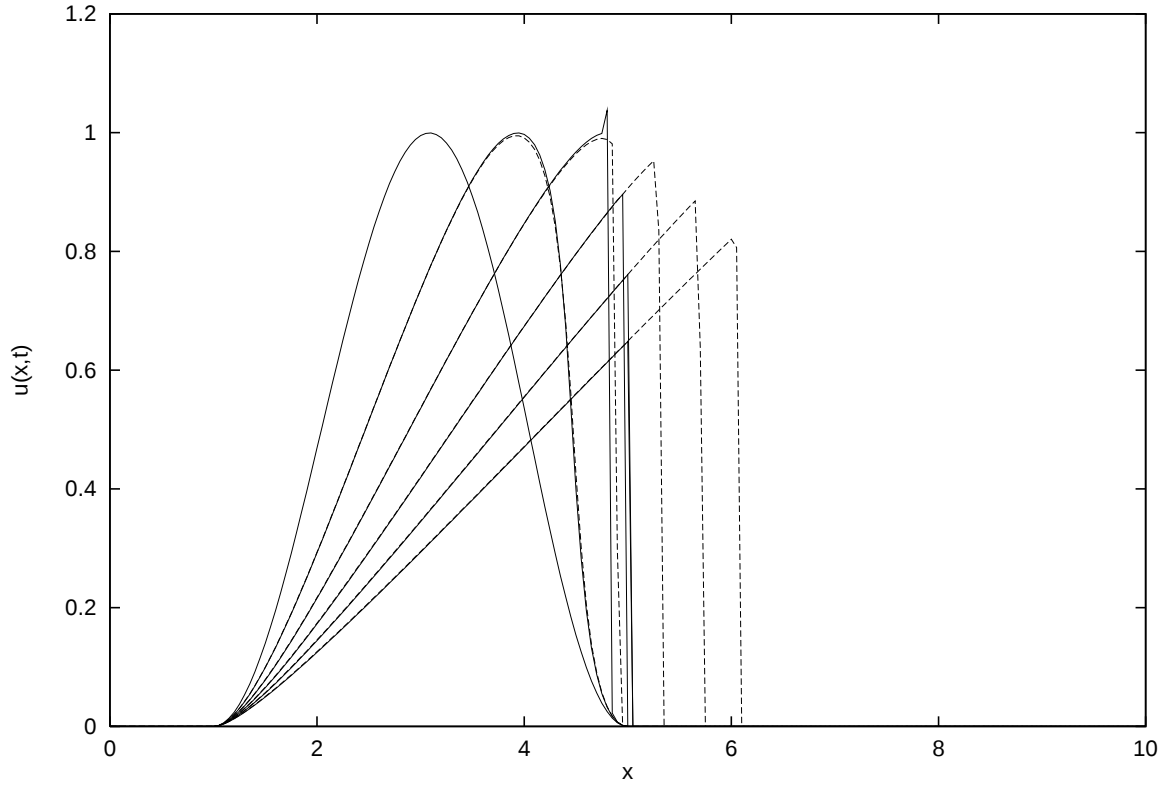
Figure 7.2: Solution of inviscid Burgers' equation using standard SL scheme: as Figure 7.1 except u_{\min} = 0 in initial data.
