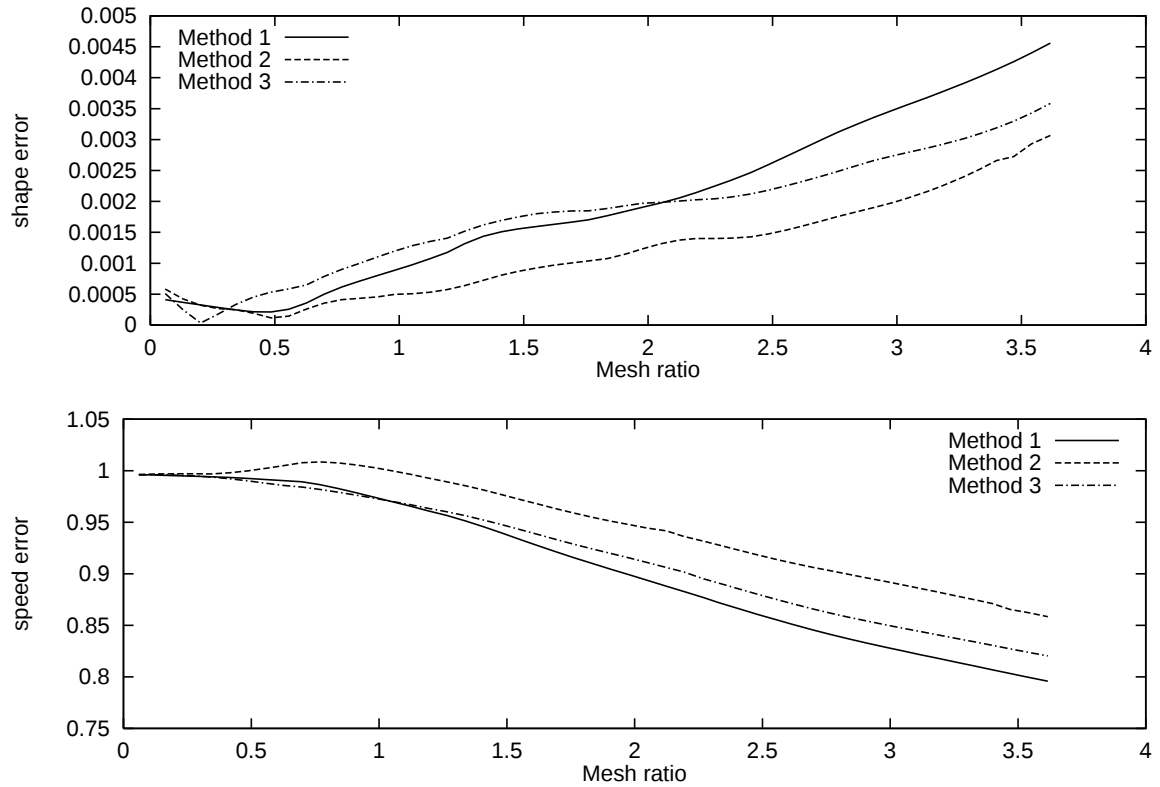
Figure 7.11: Error in speed of front and error in shape of front plotted against mesh ratio, for three different methods of calculating departure points.
