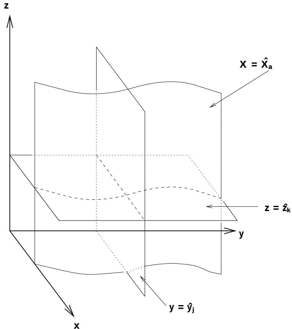
Figure 5.1: Hybrid Grids
