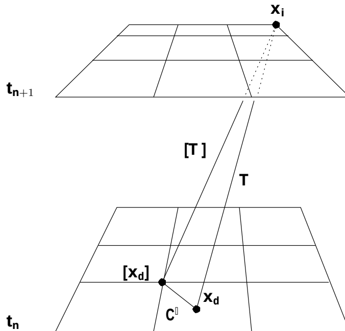
Figure 6.2: Contour Decomposition
