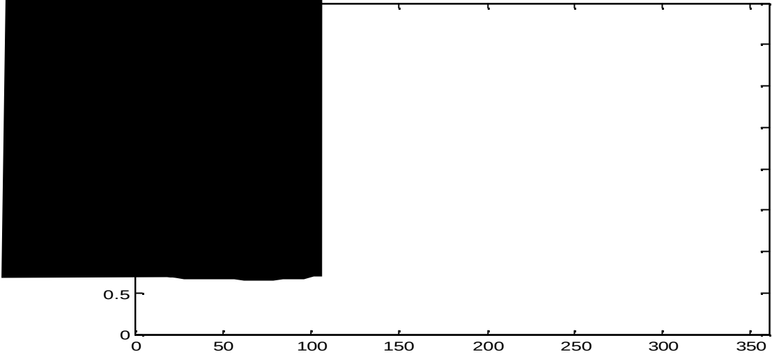
Figure 3: The HLL Scheme with the minmod limiter applied to (3)
