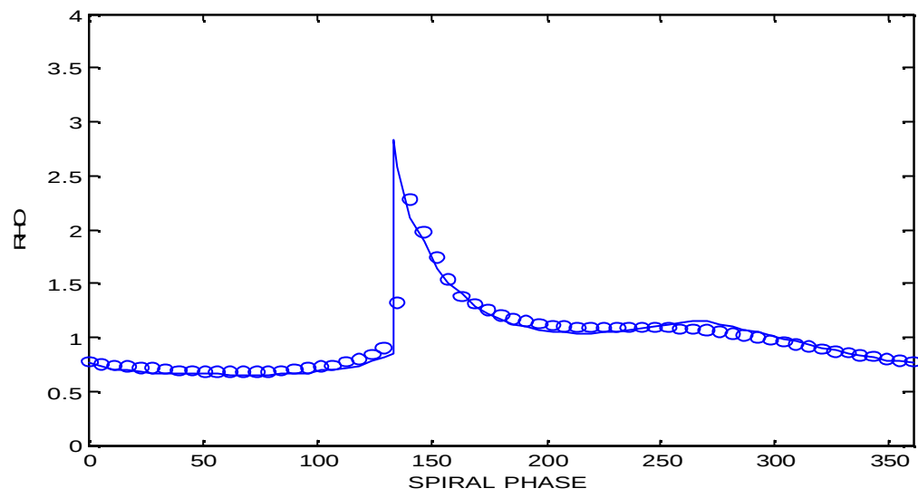
Figure nineteen: Results from the HLLC Scheme with wave speed algorithm (2)
