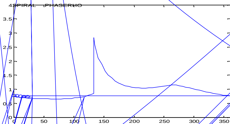
Figure five: Results from Roe's scheme with Van Leer limiter applied to the contact field and minmod applied elsewhere.
