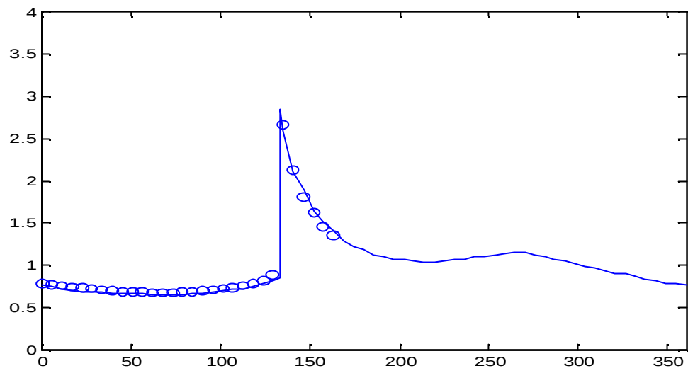
Figure six: Results from Roe's scheme with superbee applied to the contact field and minmod applied elsewhere.
