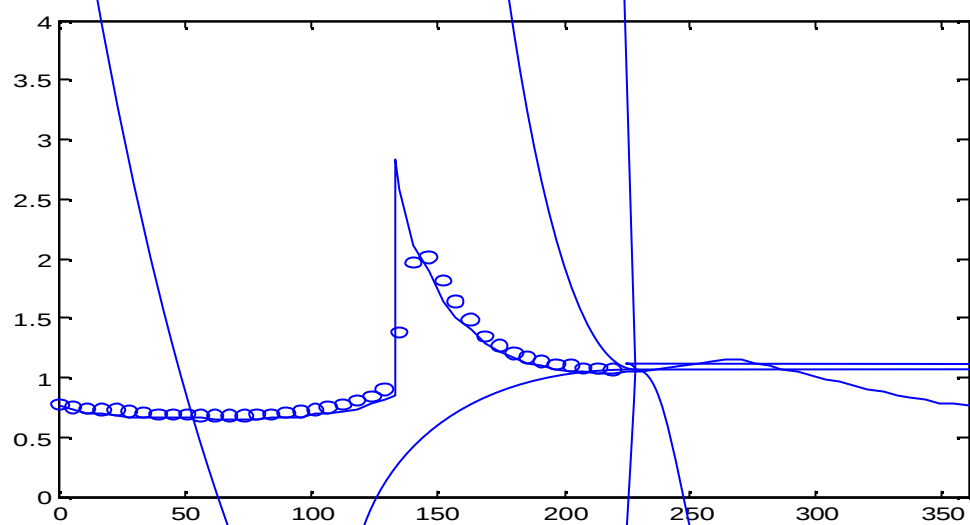
Figure thirteen: Results from the HLL Scheme with wave speed algorithm (2)
