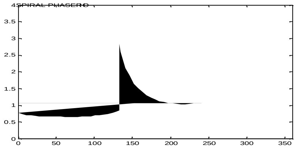
Figure one: Result's from MacCormack's method
