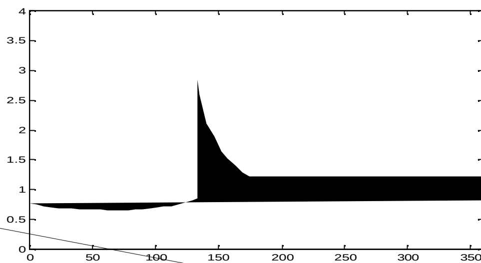
Figure three: Results from Roe's Scheme
