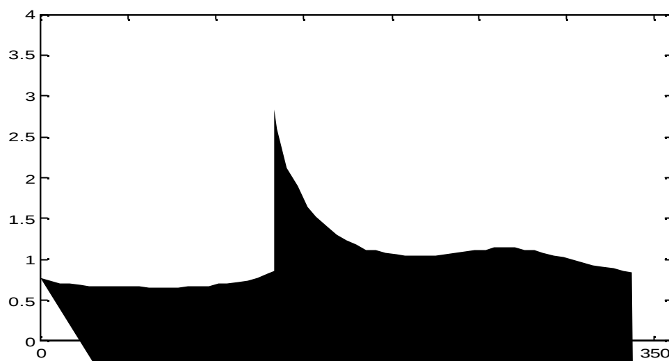
Figure twenty-two: Results from the HLLC Scheme with the superbee limiter applied to the contact field, minmod applied elsewhere and using wave speed algorithm (3)
