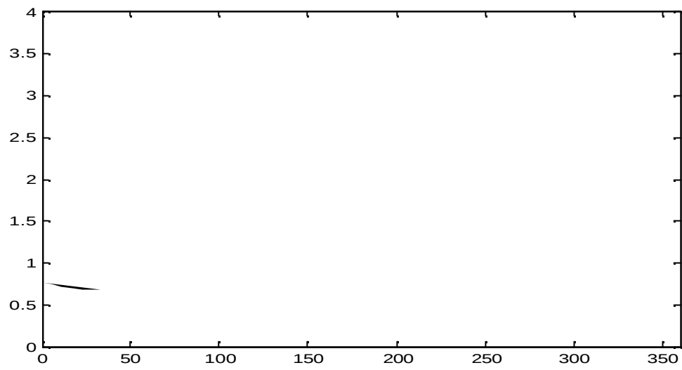
Figure nine: Results from Roe's scheme with the source term decomposed and MC limiter applied
