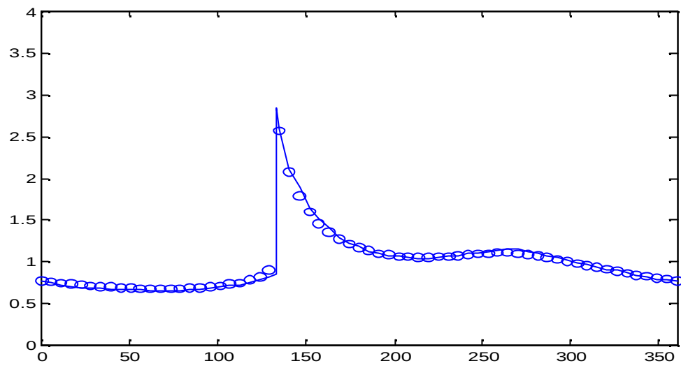
Figure eight: Results from Roe's scheme with the source term decomposed and minmod limiter applied.
