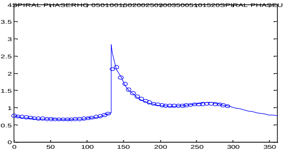
Figure seven: Results from Roe’s scheme with the source term decomposed
