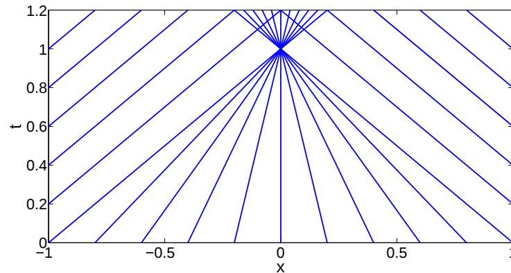
Figure 2.1: Characteristics crossing after time t = 1 causing the solution to become multivalued. This is not a physically valid solution to the problem (2.16)-(2.18).
